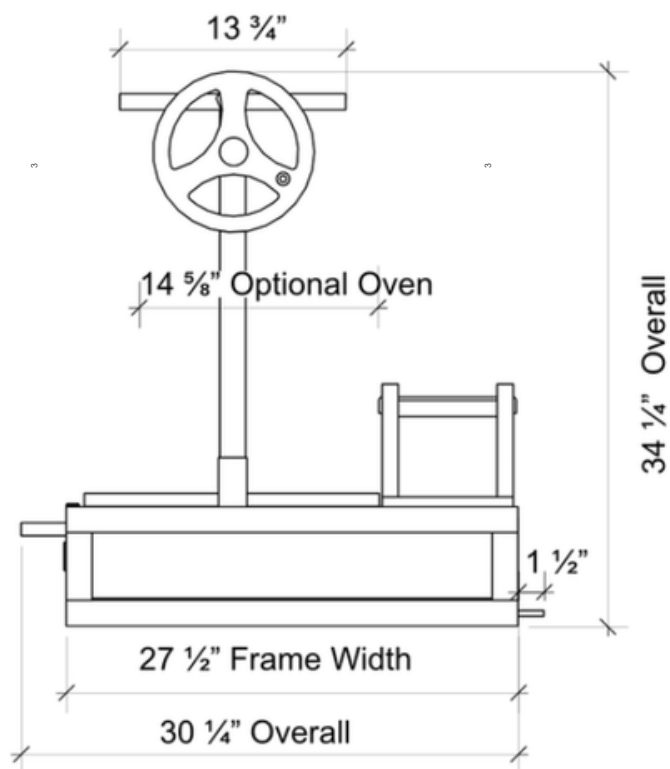
3 SIDE VIEW 1:10
