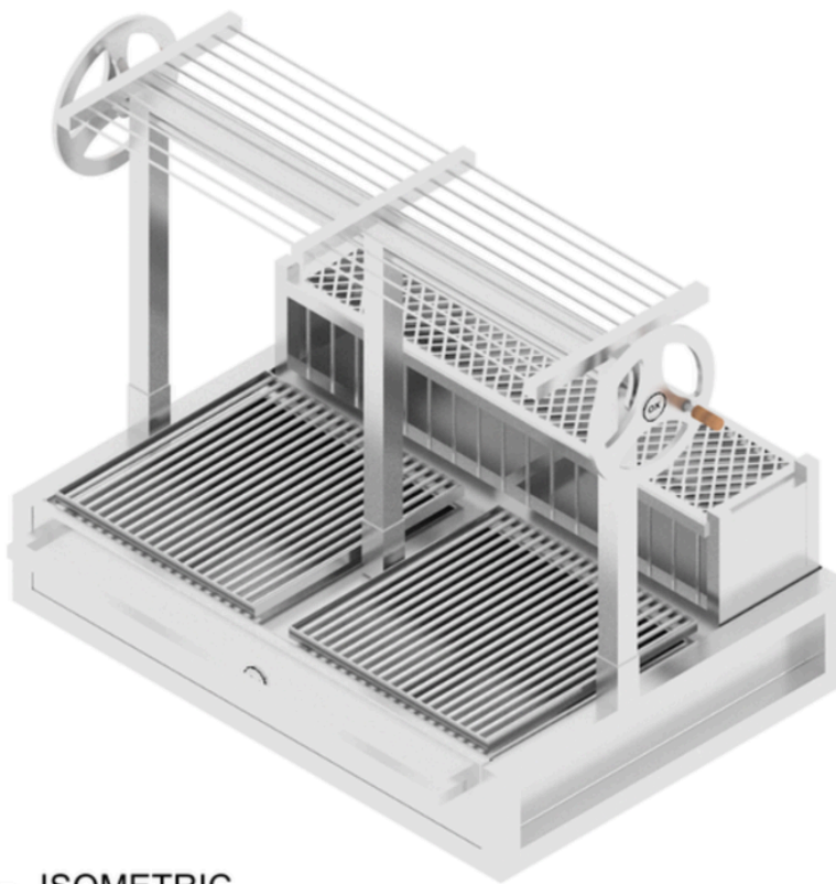
④ ISOMETRIC 1:10
